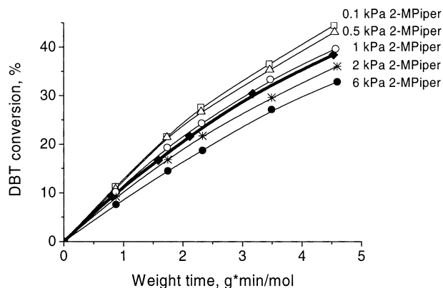
Figure 3. Total conversion of 1 kPa DBT at 300 °C and different 2-methylpyridine partial pressures. The heavy line represents the results for DBT alone.
