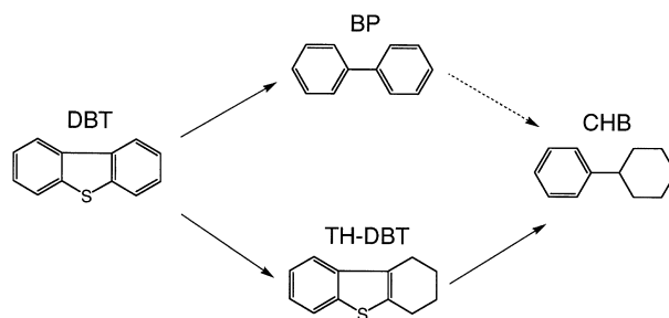
Scheme 2. Reaction network of the HDS of dibenzothiophene.
